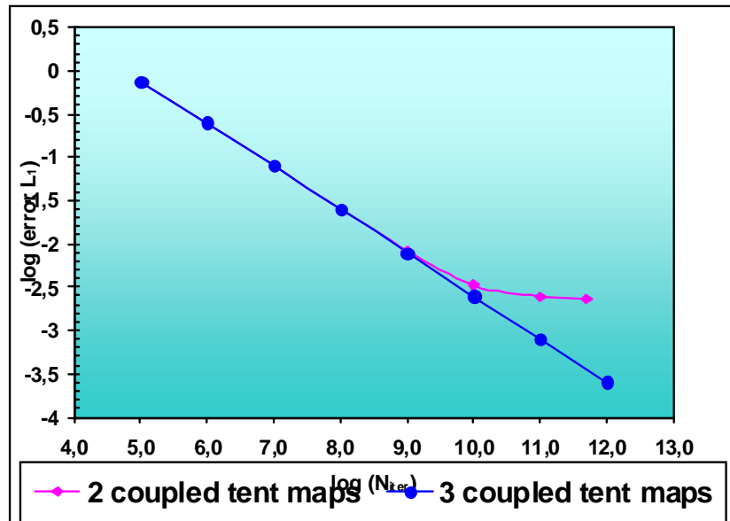
Figure 2. Error E_{1, N_{disc}, N_{iter}}(x^1) for 2 and 3-coupled symmetric tent map, double precision, N_{disc} = 10^5 , \varepsilon_1 = 10^{-14} , \varepsilon_2 = 2\varepsilon_1 , N_{iter} = 10^5 to 10^{12} . Initial values x_0^1 = 0.330 , x_0^2 = 0.3387564 , x_0^3 = 0.331353429 .
