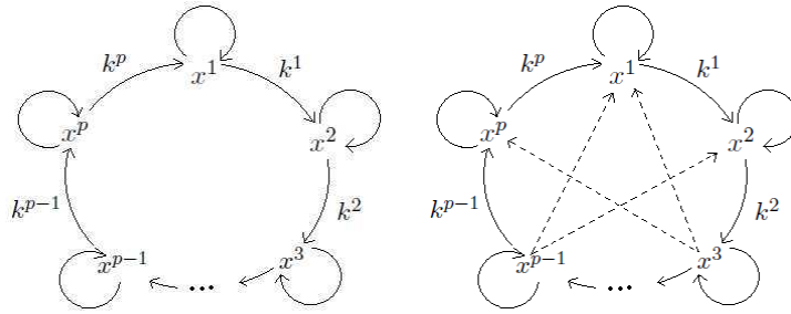
Figure 3a (left). Ring coupling between the variables x^j .
