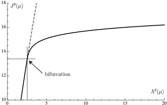
Figure 8. Parametric plot of \mu \mapsto (\Lambda^\theta(\mu), J^\theta(\mu)) for p = 3.15, d = 5, \theta = 0.95 . The behavior of the non-symmetric branch is still similar to the one found in Fig. 4.
