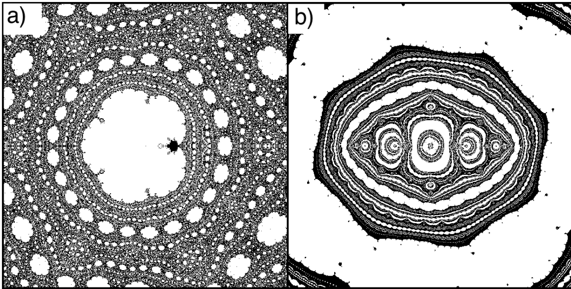
FIGURE 11: a) The bifurcation locus for the family f_\lambda with |\lambda| \approx 10^{-2} b) A Persian carpet: J(f_\lambda) with \lambda \approx 10^{-3}
