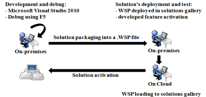
Fig. 3. The process of deploying a sandboxed solution on SharePoint Online
