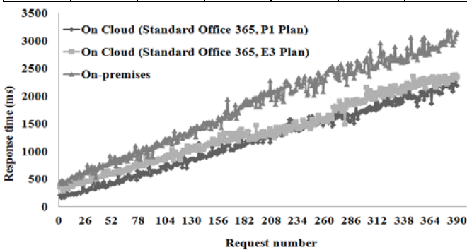
Fig. 4. Response time evolution on-premises versus on Cloud
