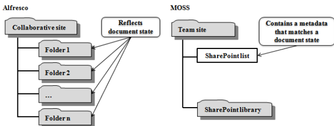
Fig. 2. Structure used to implement the documents approval Workflow
