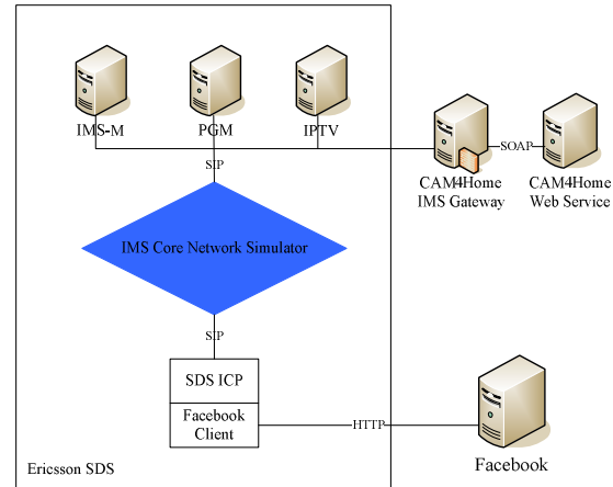
Fig. 3. Prototype system
