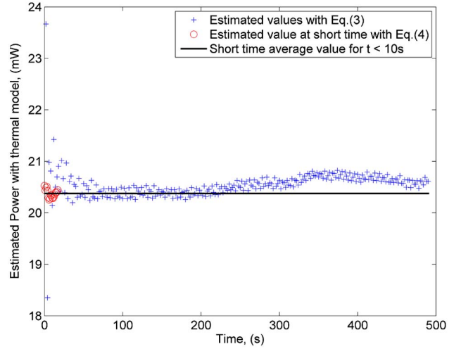
Fig. 6. (Color online) Estimated power as function of time of a 0.11 THz Gunn diode using the thermal self-calibrated model.
