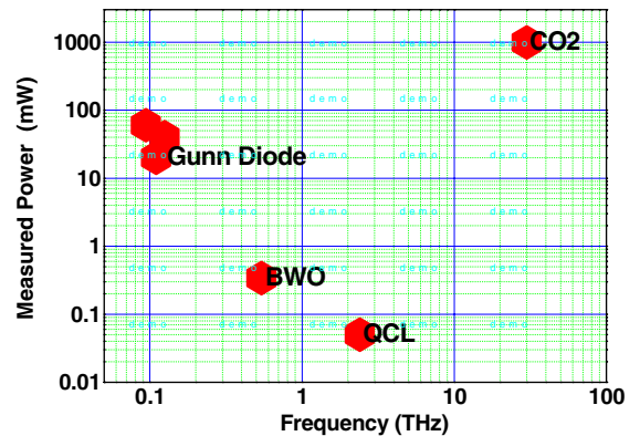
Fig. 7. (Color online) Experimental results obtained for various THz sources going from 0.1 to 30 THz with power ranging from 0.05 to 1000 mW.
