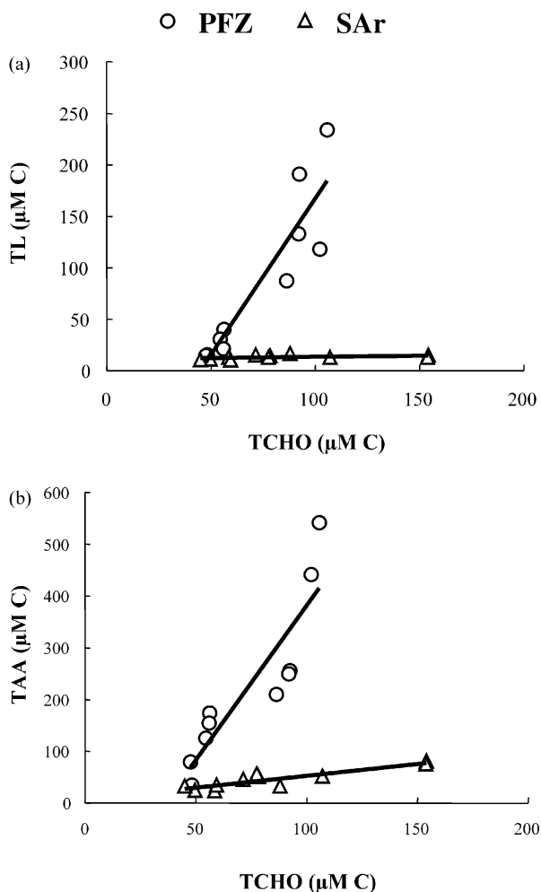
Fig. 6. Concentrations ( \mu\text{M C} ) of total lipids (a) and amino acids (b) versus total sugars in the time series samples during biodegradation experiments performed in PFZ and SAR. For each regression line from 30 and 200 m experimental data are pooled. Each regression line is described as follows: PFZ: \text{TL} = 3 \times \text{TCHO} - 136 ; r = 0.91 ; P < 0.001 ; n = 10 ; SAR: \text{TL} = 0.02 \times \text{TCHO} + 11 ; r = 0.43 ; P > 0.05 ; n = 11 ; PFZ: \text{TAA} = 5.97 \times \text{TCHO} - 216 ; r = 0.89 ; P < 0.001 ; n = 10 ; SAR: \text{TAA} = 0.46 \times \text{TCHO} + 7.06 ; r = 0.90 ; P < 0.001 ; n = 11 .
