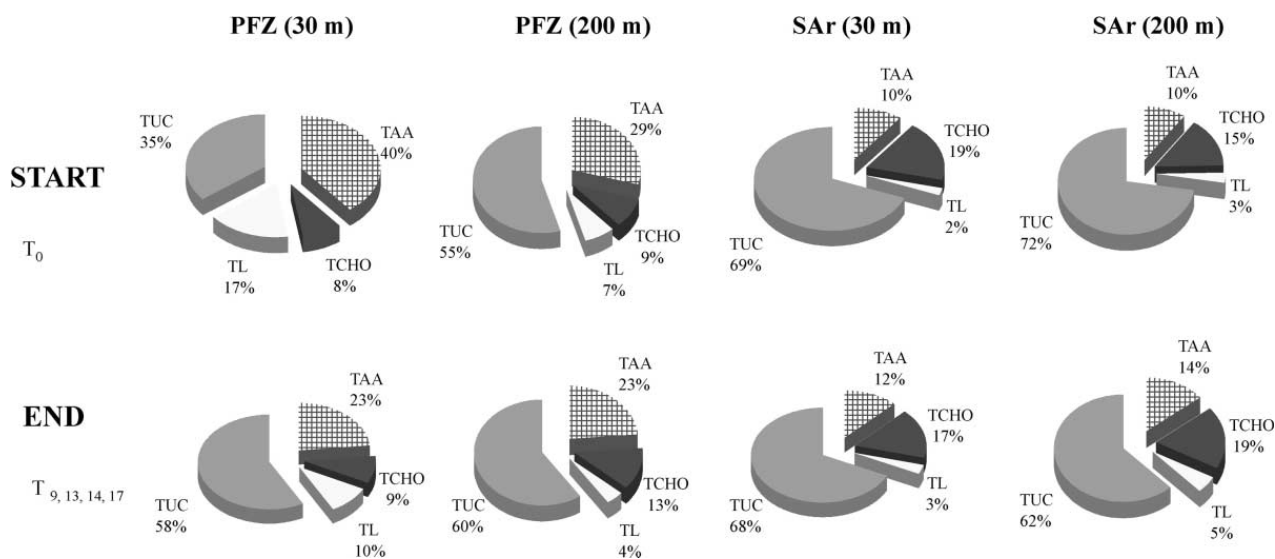
Fig. 4. Carbon contributions of characterized biochemicals to TOC at the beginning and end of the four biodegradation experiments. The fraction that could not be attributed to the amino acids, sugars and lipids is indicated as uncharacterized carbon (TUC). TUC was calculated as the difference between TOC and the sum in TAA-C + TCHO-C + TL-C.
