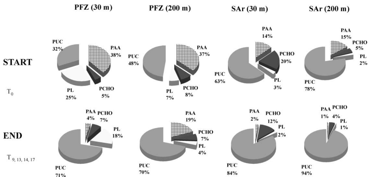
Fig. 5. Carbon contributions of characterized biochemicals to POC at the beginning and end of the four biodegradation experiments. The fraction that could not be attributed to the amino acids, sugars and lipids is indicated as uncharacterized carbon (PUC). PUC was calculated as the difference between POC and the sum in PAA-C + PCHO-C + PL-C.
