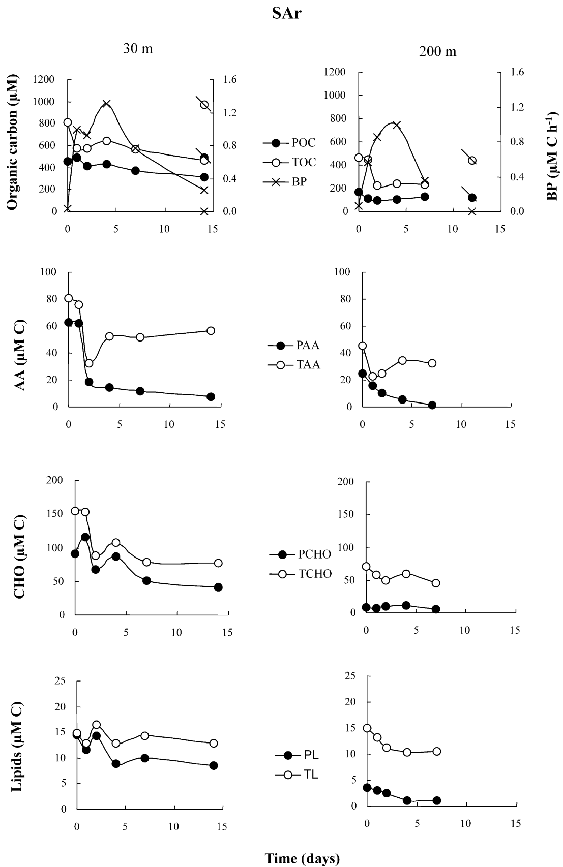
Fig. 3. Time course responses of particulate and total fractions of organic carbon, amino acids, sugars and lipids in relation to bacterial production during biodegradation experiments at SAr 30 m and 200 m depth. Same abbreviations as in Fig. 2.
