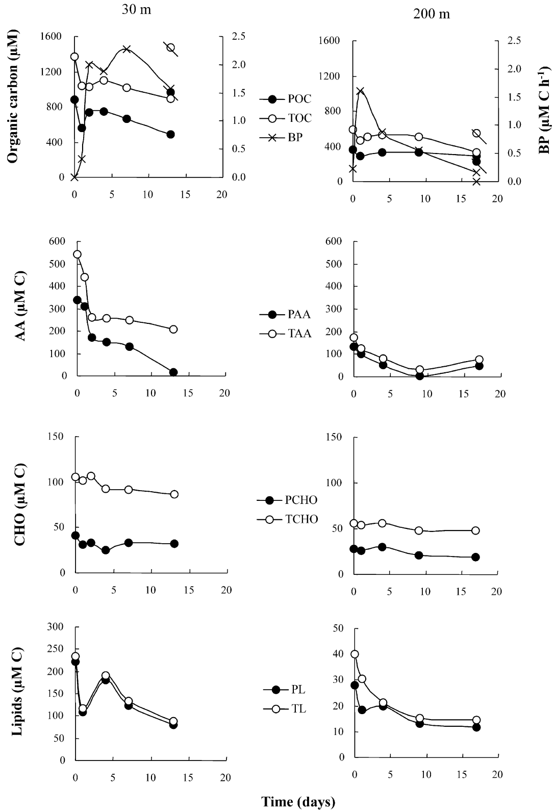
Fig. 2. Time course responses of particulate and total fractions of organic carbon, amino acids, sugars and lipids in relation to bacterial production during biodegradation experiments at PFZ 30 m and 200 m depth. Dots with slash represent control experiments for POC and TOC.
