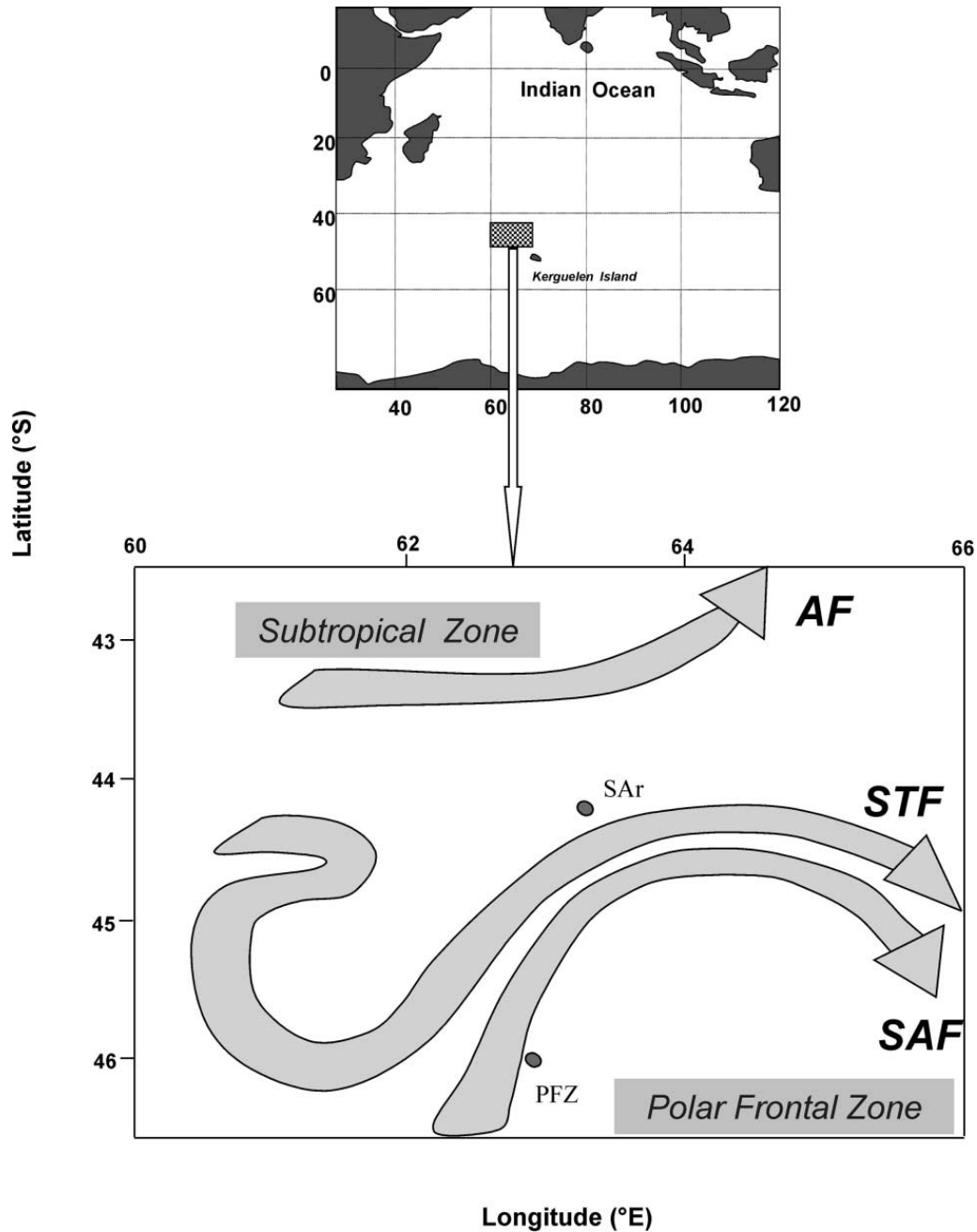
Fig. 1. Locations of stations during the cruise Antares 4 in the Southern Ocean (January–February 1999). Notations: Agulhas Return Front (AF), Sub-tropical front (STF), Sub-antarctic Front (SAF).
