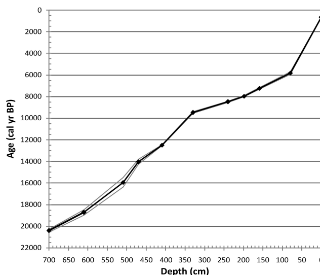
Fig. 2. Age–depth model for core MD04-2797CQ. Grey lines indicate the 1 \sigma error envelope.
