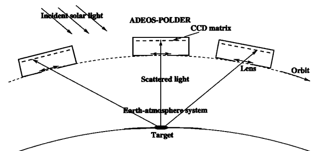
Figure 8. Viewing geometry of ADEOS-POLDER.
