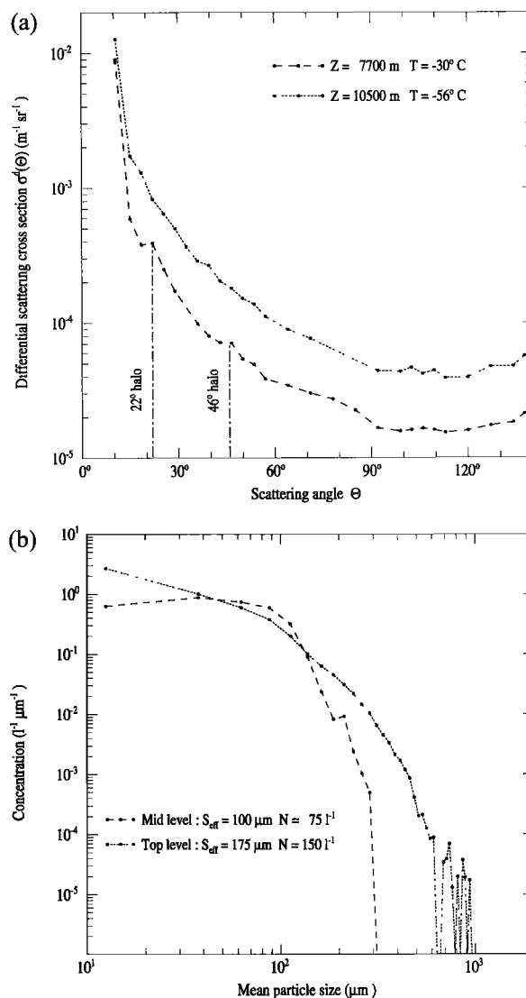
Figure 6. (top) Polar nephelometer measurements and (bottom) corresponding particle size distribution from PMS OAP-2D2-C probe.
