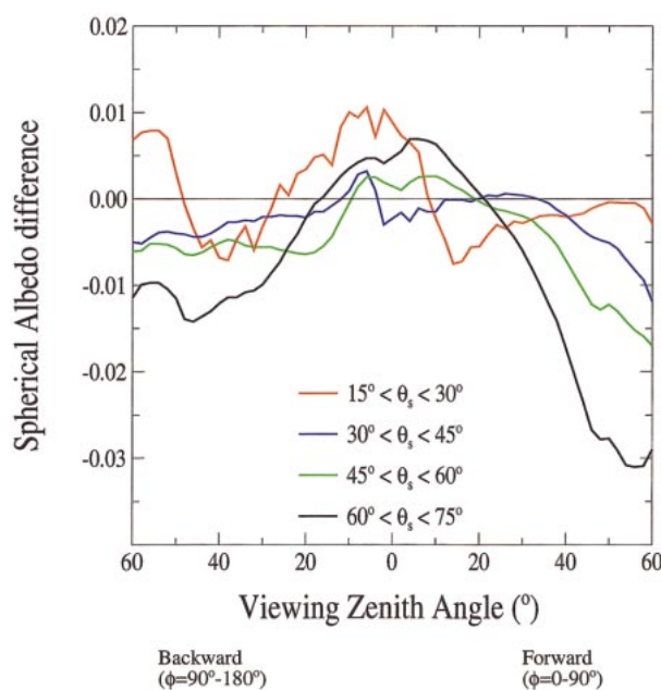
FIG. 6. Cloud spherical albedo difference S_{10}(\Theta) - S_{10}(120^\circ) as a function of viewing zenith angle \theta_v , for the whole dataset by classes of solar zenith angle.
