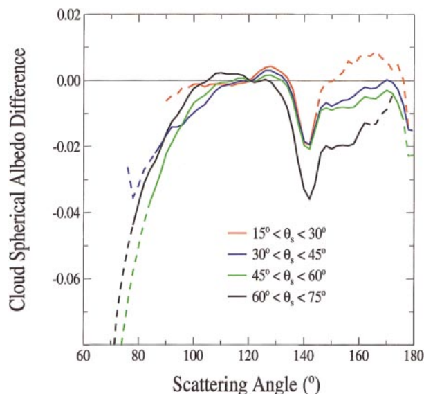
FIG. 5. As in Fig. 4 but for the whole dataset by classes of solar zenith angle.
