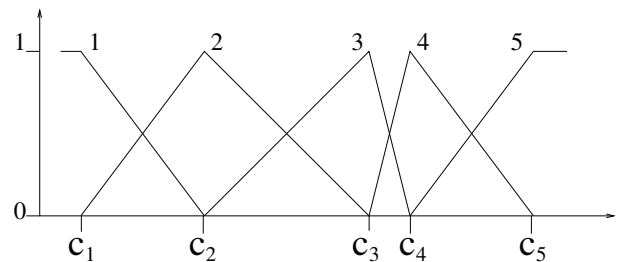
Fig. 2. A five linguistic strong fuzzy partition
