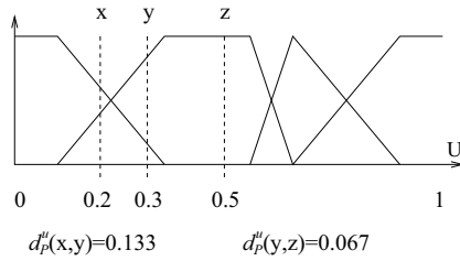
Fig. 8. Example of fuzzy partition based distance behavior( d_p^u )
