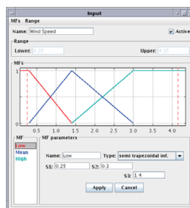
Fig. 2. A strong fuzzy partition
