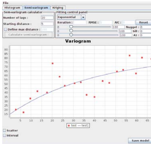
Fig. 6. GeoFIS variogram window
