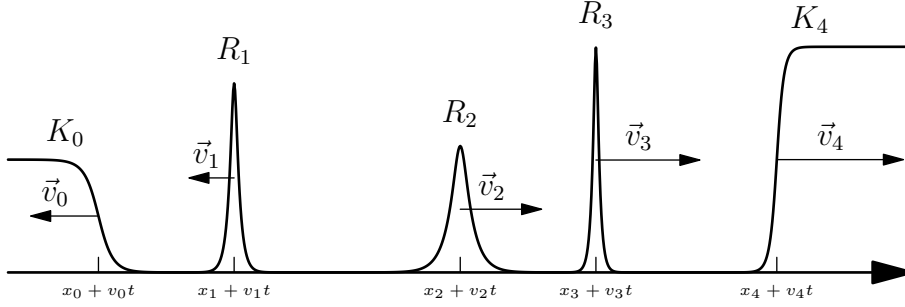
Figure 1: Schematic representation of the multi-kink profile KR in (1.21)
