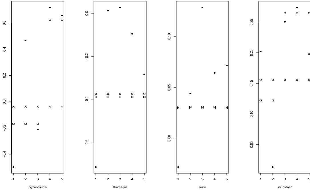
Fig. 1. Estimates for the bladder data in the multiplicative model. The crosses represent the constant estimator, the filled circles the unconstrained estimator and the squares the reweighed lasso estimator.
