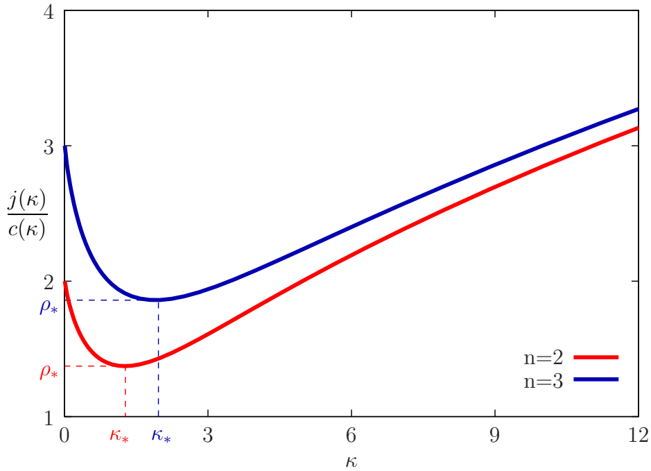
Figure 2: The function \kappa \mapsto \frac{j(\kappa)}{c(\kappa)} , in dimensions 2 and 3.
