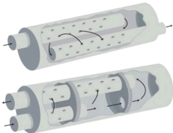
Image 12: Internal View of Reactive Attenuator
