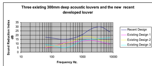
Graph 3: Improvement of new design over standard
