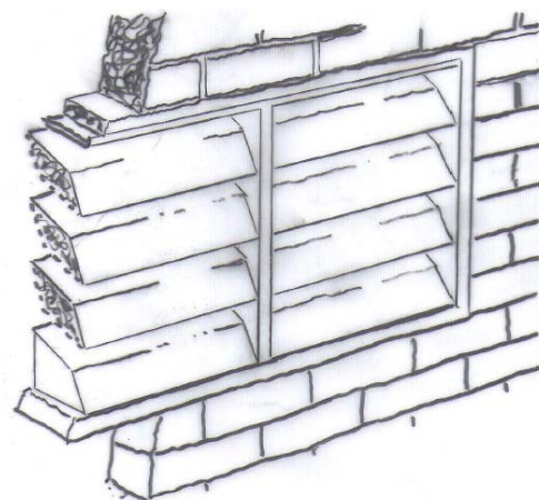
Image 10: Layout for Standard Acoustic louver
