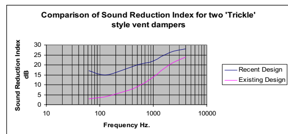
Graph 4: Improvement of new design over standard
