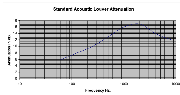
Graph 2: Attenuation offered by Louver
