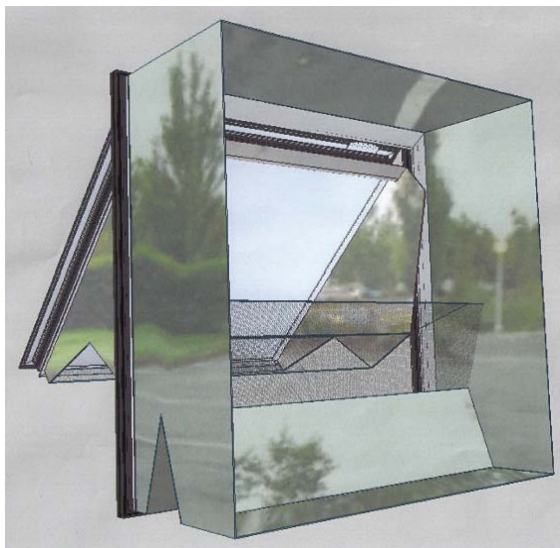
Image 3: 'Trickle Vent' Damper / Attenuator
