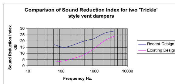
Graph 4: Improvement of new design over standard
