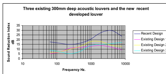
Graph 3: Improvement of new design over standard
