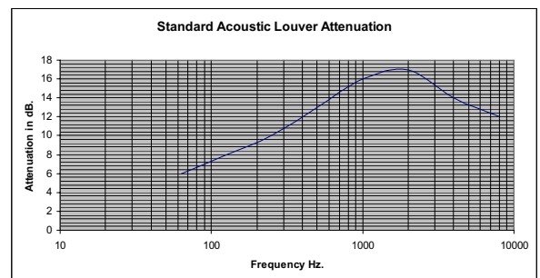
Graph 2: Attenuation offered by Louver
