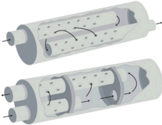
Image 12: Internal View of Reactive Attenuator
