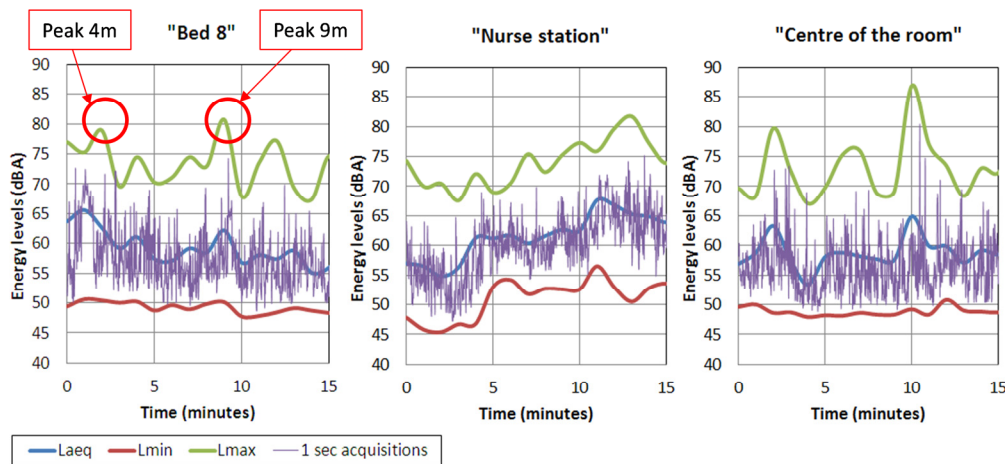
Figure 5: Energetic levels for three locations relative to 1 minute time intervals (initial 15 minutes). The plots also show the relative 1-second L_{Aeq} values, for comparison.
