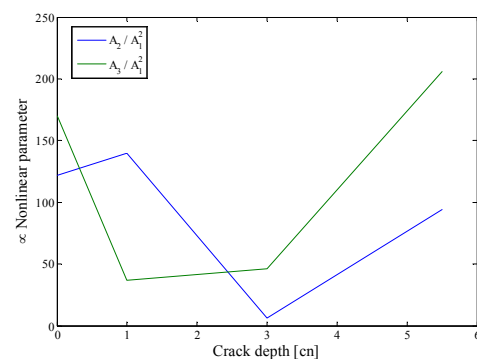
Figure 5 : Evolution of the nonlinear parameters \alpha and \beta (arbitrary unit) with the depth of the crack
