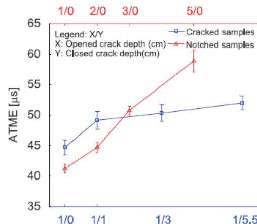
Figure 8 : Evolution of the ATME with the notch depth (red) or the crack depth (blue)
