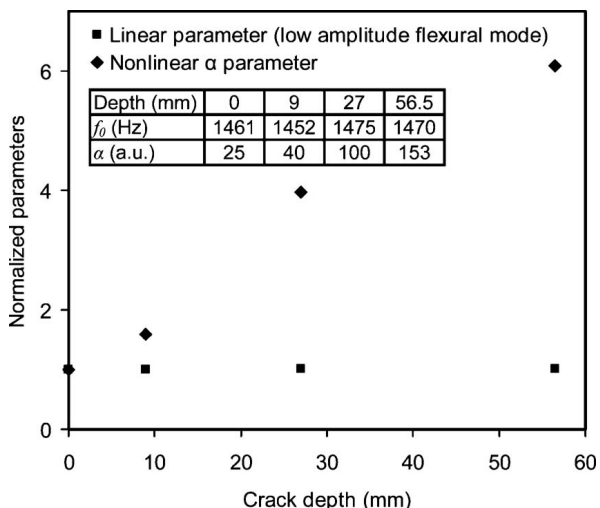
Figure 9 : Evolution of the nonlinear (arbitrary unit) and linear parameters with the depth of the crack
