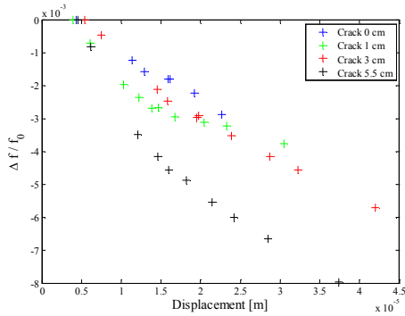
Figure 6 : Evolution of the resonance frequency gap with the displacement amplitude.
