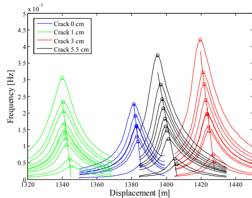
Figure 4 : Curve indicating frequency gap for NRUS cracked samples with various depths (0, 1, 3, 5.5 cm)
