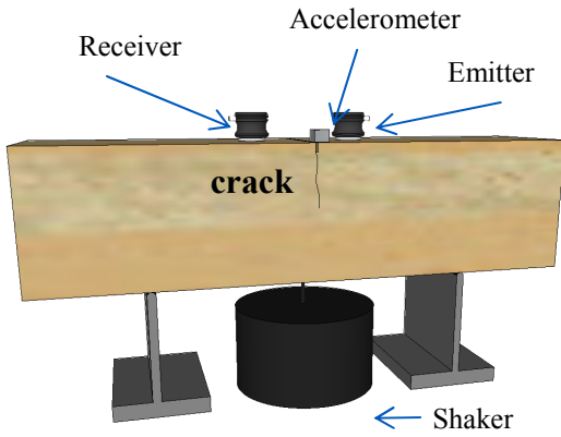
Figure 2 : Assemblage for testing on a concrete beam
