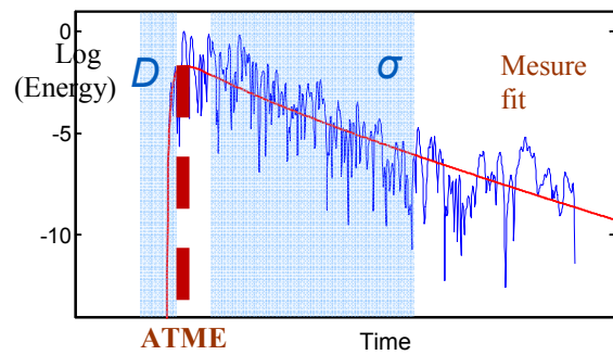
Figure 7 : Smoothing (unbroken line) of the evolution of the energy transported by the signal as a function of the time by a 2D solution [21] of equation (5)
