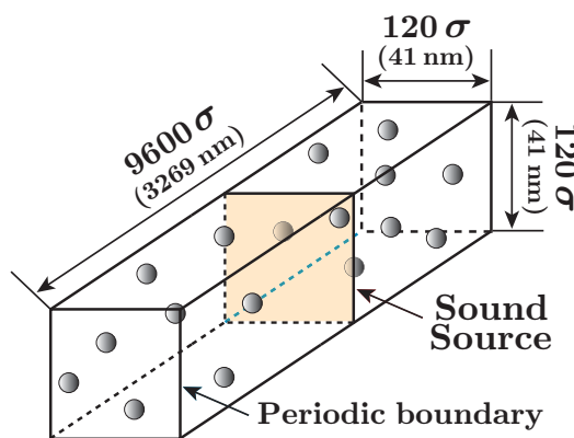
Figure 2: Simulation box and sound source.
