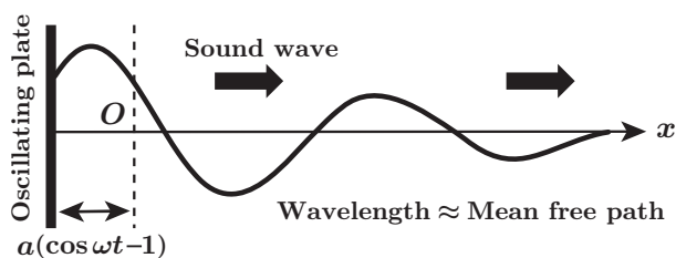
Figure 1: Schematic of model.
