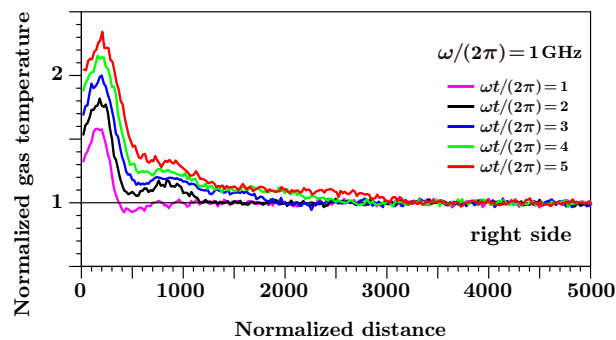
Figure 5: Temperature elevation in the gas.
