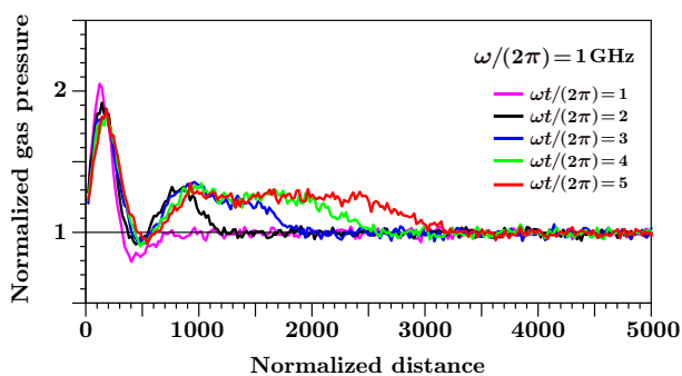
Figure 3: Profile of gas pressure in a large-amplitude progressive sound wave with frequency 1 GHz.
