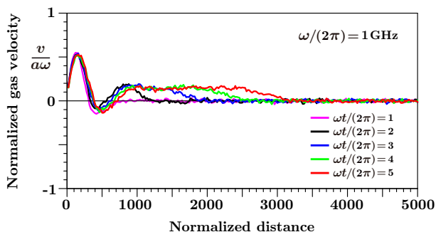
Figure 4: Profile of gas velocity in a large-amplitude progressive sound wave with frequency 1 GHz.
