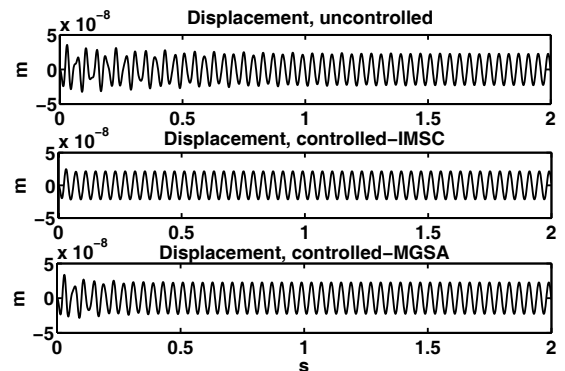
Figure 4: IMSC/ MGSA time response comparisons for harmonic excitations
