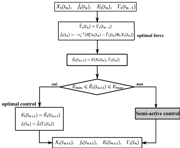
Figure 1: Algorithm of modal global semi-active control
