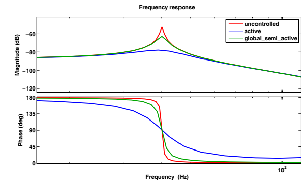
(b) Zoom of the first mode frequency response
