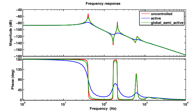
(a) Frequency response of the beam: IMSC(dashed) /MGSA (dotted) comparisons
