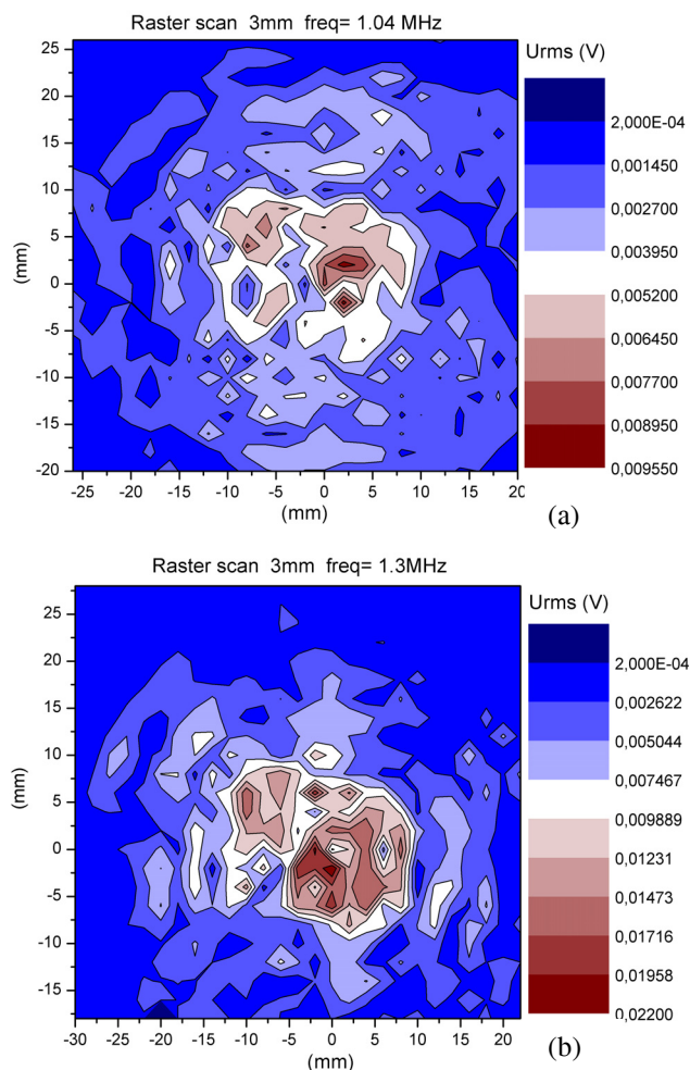
Figure 3: Comparison of raster scans at 0.3 cm for a) 1.040 MHz and b) 1.320 MHz.
