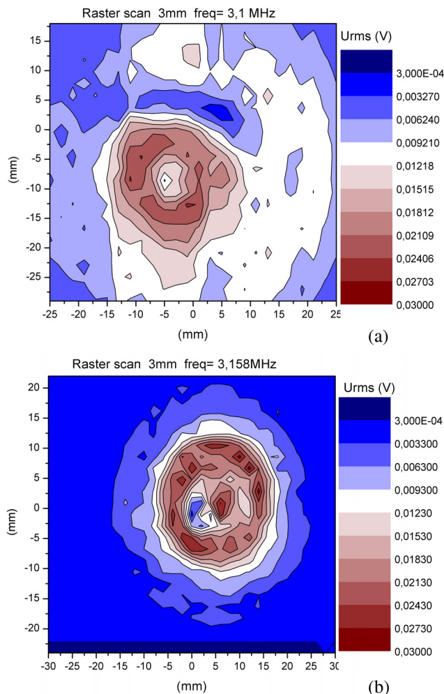
Figure 6: Comparison of raster scans at 0.3 cm for a) 3.1 MHz and b) 3.158 MHz.
