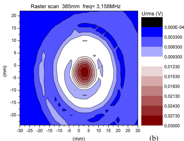
Figure 5: Raster scan performed in two planes orthogonal, at z = 0.3 cm from the transducer (a), at z_N = 38.5 cm (b), at the working frequency = 3.158 MHz.
