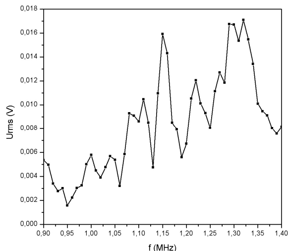
Figure 1: Transducer 1 MHz: frequency response, in z_N .
