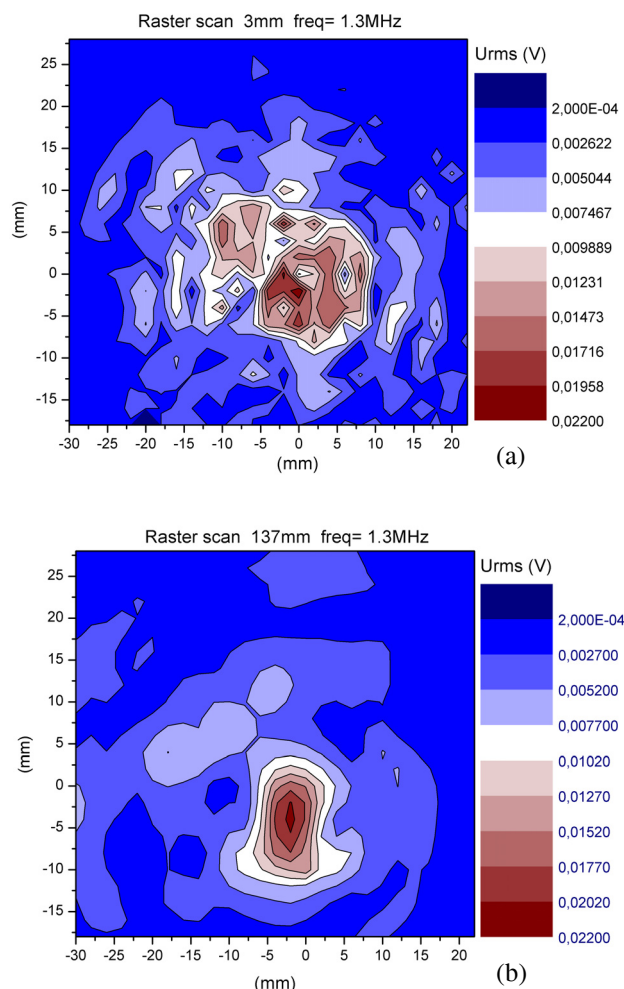
Figure 2: Raster scan performed in two planes orthogonal, at z = 0.3 cm from the transducer (a), at z_N = 13.7 cm (b), at the working frequency = 1.320 MHz.
