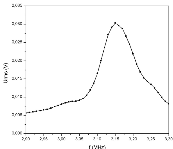
Figure 4: Transducer 3 MHz: frequency response, in z_N .
