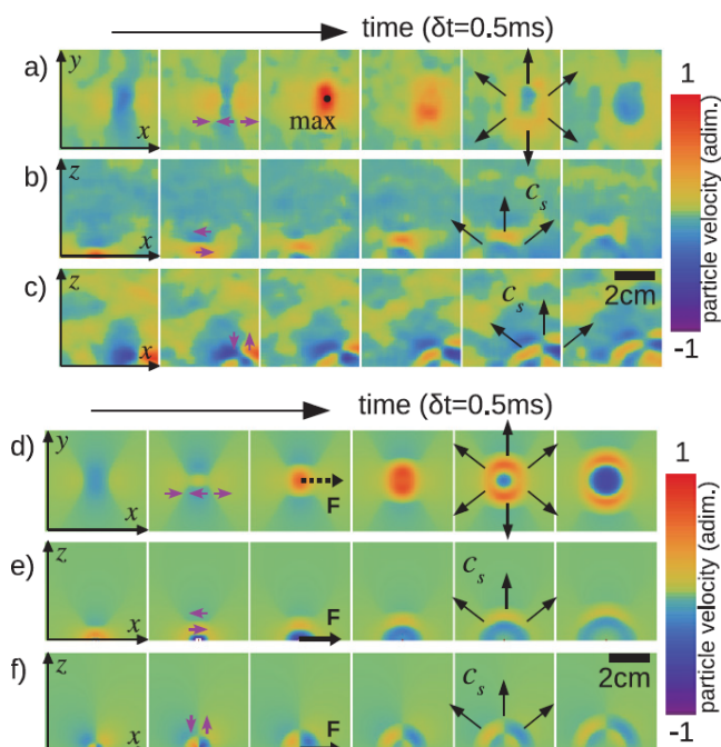
Figure 2: Left part: experimental observations of events occurring during friction between the gel and the sandpaper. (a) Observation along the plane P1 of the component v_x . (b) Observation along the plane P2 of the component v_x . (c) Observation along the plane P2 of the component v_z . The images areas are 4.5\times 4.5\text{ cm}^2 and the time-step is 0.5 ms between each frame. The amplitudes are normalised to get a maximum of 1 on each line. Many similar events are observed, with variable amplitudes but same radiative pattern. Right part: Green function computation gives the theoretical response of the gel submitted to a horizontal punctual and temporally Gaussian force applied at the interface 0.5ms before first frames in the x -direction (represented by F in third frames). (d) plane P1, v_x ; (e) plane P2, v_x ; (f) plane P2, v_z . The purple arrows materialise the direction of the imaged component in each case.
