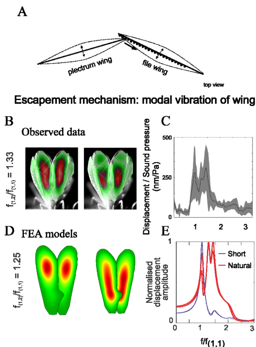
Figure 2: The function of resonance in tree cricket wings. (A) A cartoon of the cricket singing escapement mechanism. (B) A vibrometric map of displacement of tree cricket wings at model (1,1) and mode (1,2). (C) Amplitude spectra of wing displacement, mean and standard deviation as measured at the harp area. (D) FE models of stiff isotropic plates shaped like wings at mode (1,1) and mode (1,2) and (E) the frequency response of these plates with measured damping parameters included.
