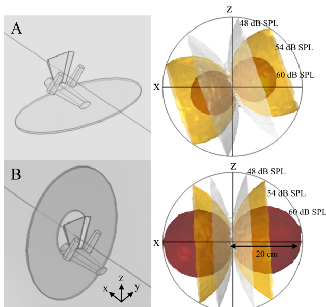
Figure 3: The effect of a baffle on sound radiation.
