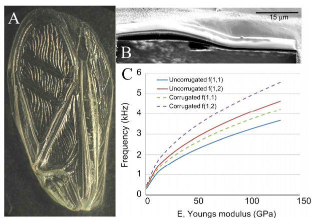
Figure 5: Effects of wing corrugation (A) Wing of O. henryi male. Corrugations are clearly visible on flat wing areas. (B) SEM through a corrugation on the harp. (C) Eigenfrequencies, f_{(1,1)} and f_{(1,2)} in corrugated and uncorrugated wings their relationship with the wings bulk Young's modulus.
