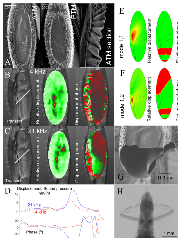
Figure 6: O. henryi auditory system. (A) The tympanal membranes, ATM and PTM of O. henryi . ATM response to sound at (B) 4 kHz and at (C) 21 kHz. (D) The amplitude and displacement of the ATM along the transect shown on (C) at these two frequencies. (E, F) First two eigenmodes of the FE models of the O. henryi ATM (G) A section through an O. henryi leg near the tympanal membranes. (H) X-ray micrograph of O. henryi auditory trachea.
