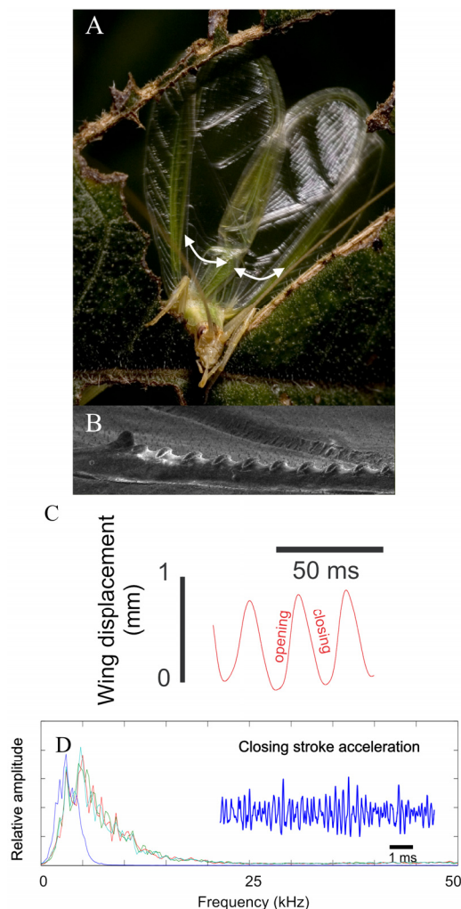
Figure 1: Singing behavior of tree-crickets. (A) A singing tree cricket. (B) SEM of O. henryi file teeth. (C) Displacement of wing during singing. (D) Acceleration during a closing stroke and frequency spectra of closing stroke accelerations of 4 individuals.
