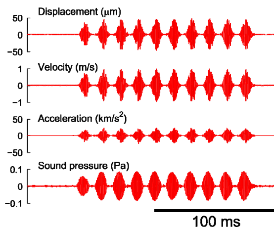
Figure 4: Wing motion and song of an O. henryi male singing from a baffle. Wing displacement, velocity and acceleration at point of maximum amplitude on the wing and simultaneous sound recording at 20 cms from animal.
