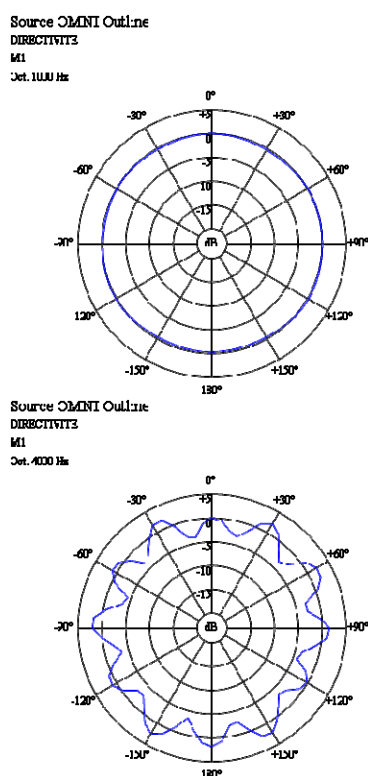
Figure 1: Polar responses of the source at 1kHz and 4kHz.
