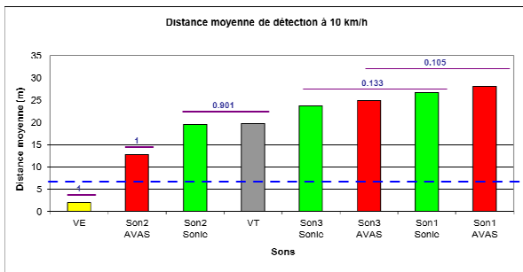
DUNCAN detection at 10km/h
