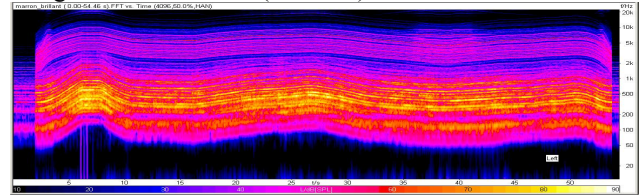
3D Time/frequency domain of sound 1
