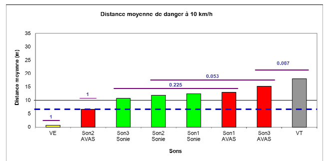
DUNCAN danger at 10km/h
