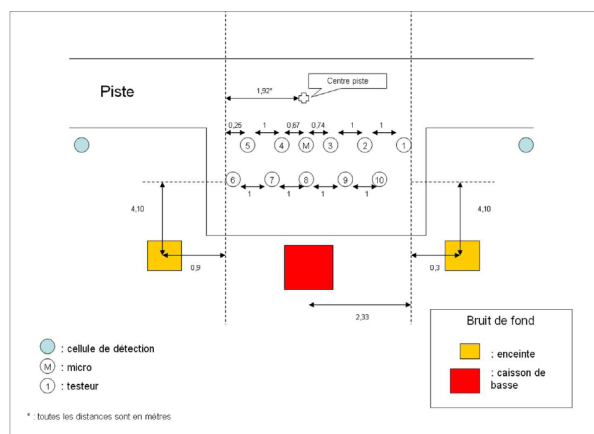
Test area disposal
