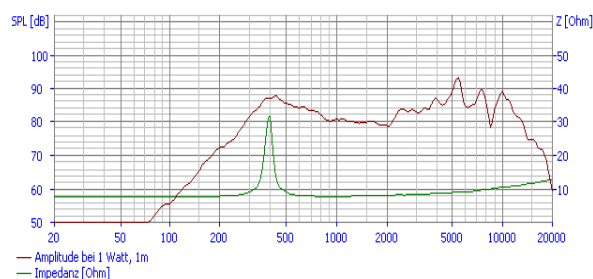
50 mm loudspeaker's characteristics
