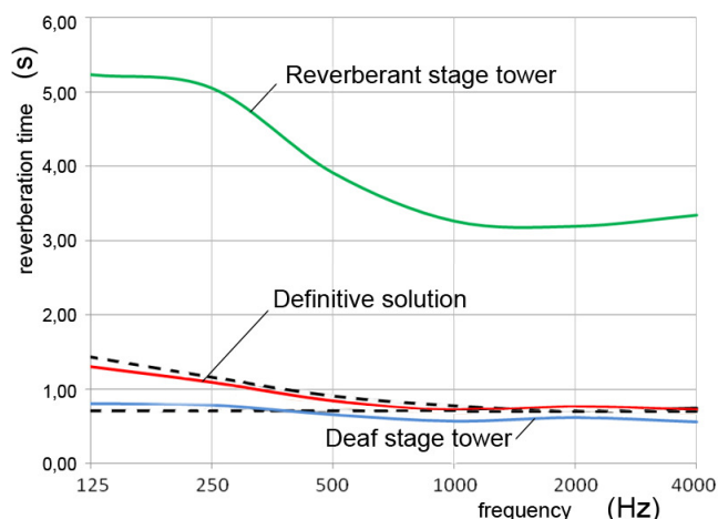
Figure 11: Trend of T_{30} , for the hall in the definitive solution (DS) and the other two. The dashed lines indicate the acceptability range for the reverberation time in the halls destined to prose performances, with a volume comparable to the one examined.
