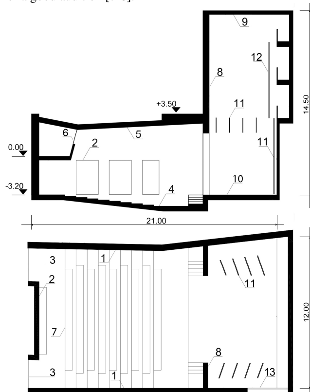
Figure 6: Plan (lower) and section (upper) of the new Theatre [3]. The numbers indicate the covering materials reported in Tab. 1.
