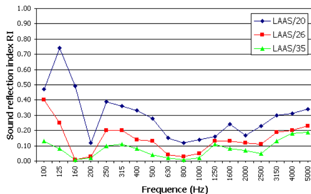
Figure 4: results of in situ measurements of sound reflection index as a function of frequency for the LAAS configurations.
