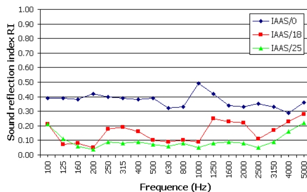
Figure 4: results of in situ measurements of sound reflection index as a function of frequency for the IAAS configurations.
