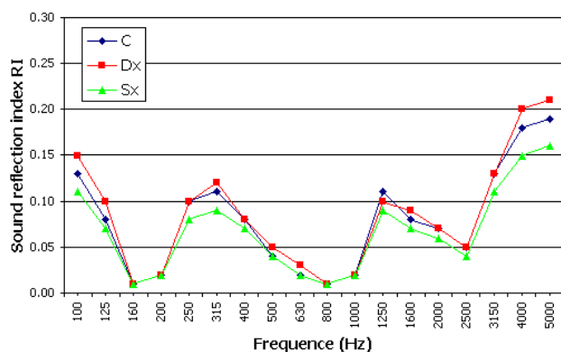
Figure 7: results of in situ measurements of sound reflection index as a function of frequency for different MSAs (LAAS/35 configuration).
