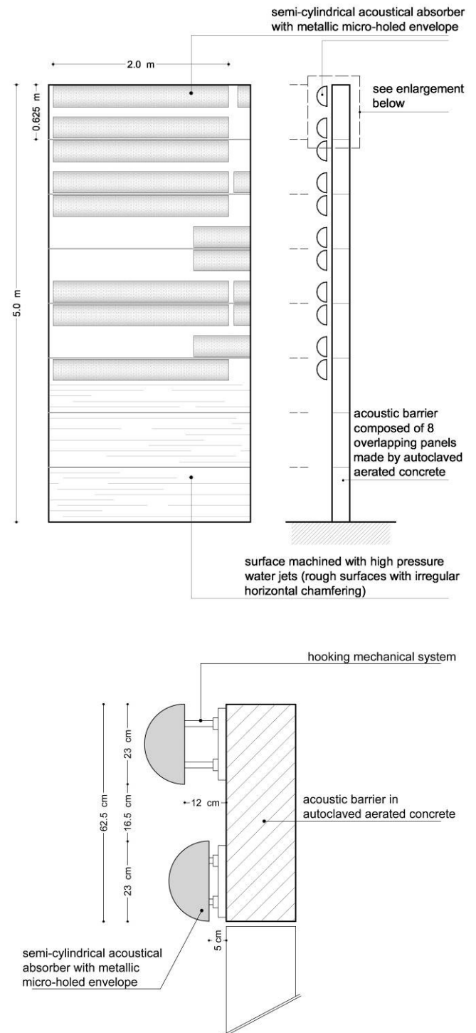
Figure 3: schematic representation of the analyzed noise barriers (top) with details of the main dimensions of the semi-cylindrical acoustical absorbers (bottom).
