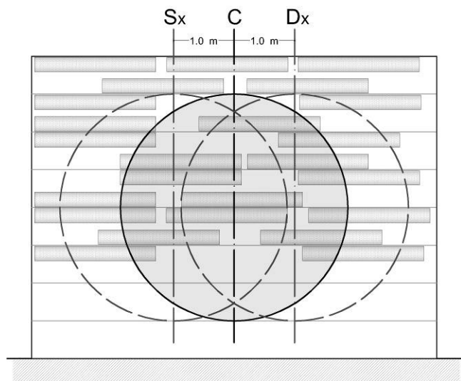
Figure 6: indication of the vertical planes used in the in situ measurements for the positioning of the complex loudspeaker-microphone and representation of the relative MSA.
