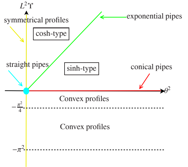
Figure 2: Categorization of profile types w.r.t. \theta and L^2\Upsilon .
