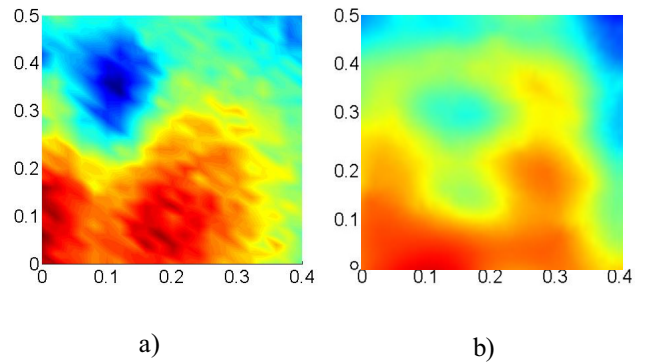
Figure 6 Sound Pressure Level distribution in an horizontal plane behind the crystal at 1000Hz for a) experimental measurements and b) numeric simulations
