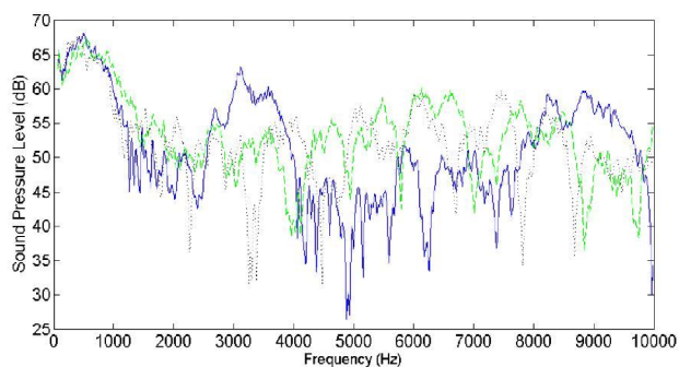
Figure 6 Sound Pressure Level spectra measured for three different positions behind the crystal in the transverse section y=-10\text{cm} (dotted), y=0\text{cm} (continuous, align with the source) and y=10\text{cm} (dashed).
