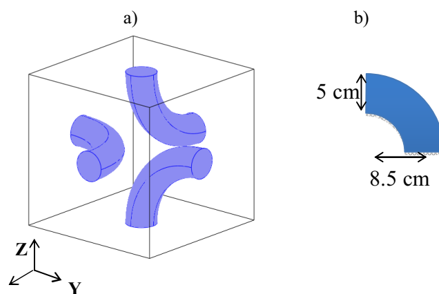
Figure 1 a) Unit cell and b) geometric dimensions of each elbow
