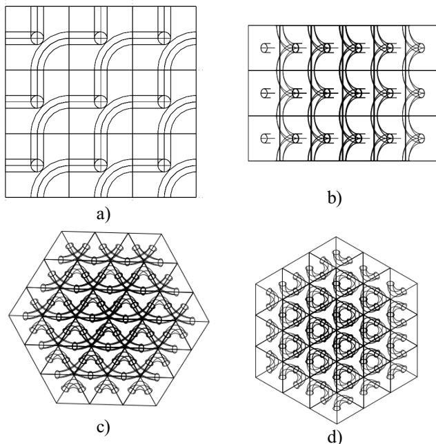
Figure 2 Different views of the Sonic crystal from directions a) [1 0 0], b) [1 1 0], c) [-1 1 1] and d) [1 1 1]
