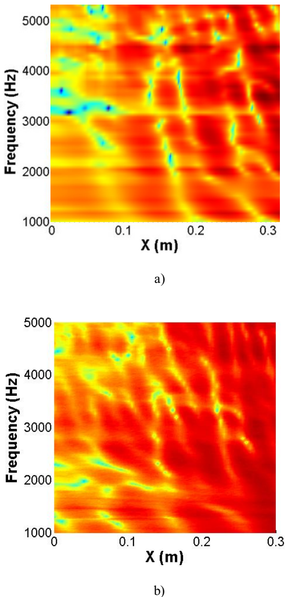
Figure 5 Sound Field inside the crystal for a) experimental measurements and b) numerical simulations
