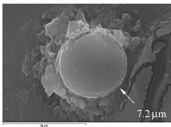
Figure 4: SEM image post mortem of the fiber cross-section close to the point of laser ultrasonic measurements. The cross-section is nearly circular with a diameter of 7.2 \mu\text{m} .
