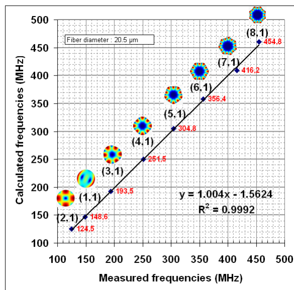
Figure 3: The best fit of the calculated frequencies with the measured frequencies (red values) giving a fiber diameter (20.5 \pm 0.4) \mu\text{m} . The modal shape of eigenmodes (m, n) are represented.
