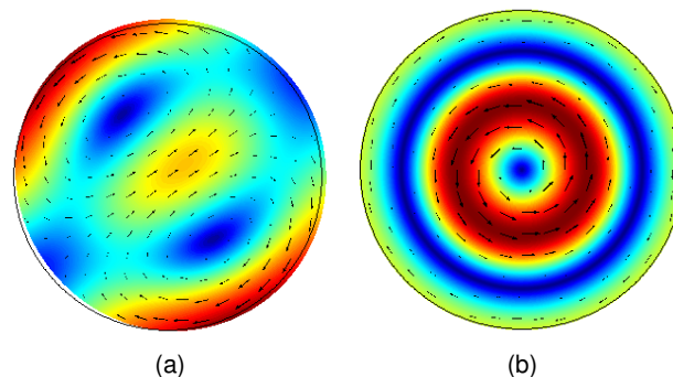
Figure 1: Display of the displacement field for two particular modes of a circular fiber. (a) The first dipolar mode: (m, n) = (1, 1) and (b) The first torsional mode: (m, n) = (0, 1) . The arrows show both the direction and magnitude of the displacement vectors. The color scale represents the magnitude of the displacement, the red color corresponds to the maximum of the displacement field and the deep blue color corresponds to nodal points.
