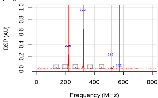
Figure 5: Vibration spectrum of a T700 carbon fiber. The vertical axis represents the power density.
