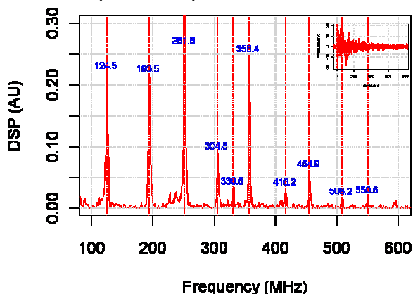
Figure 2: The vibration spectrum of a E-glass fiber. The vertical scale is the power density of the displacement signal shown in the inset.
