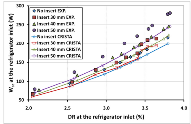
Figure 4: Evolution of the acoustic power as function as the drive ratio at the refrigerator inlet with and without the inserts between CRISTA results and experimental measurements.
