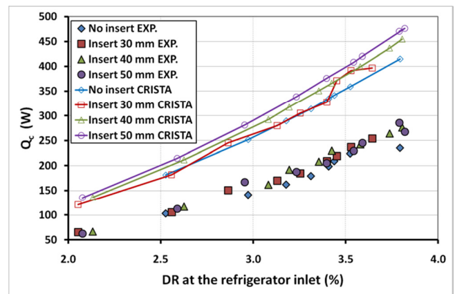
Figure 5: Evolution of the cold power as function as the drive ratio at the refrigerator inlet with and without the inserts between CRISTA results and experimental measurements.
