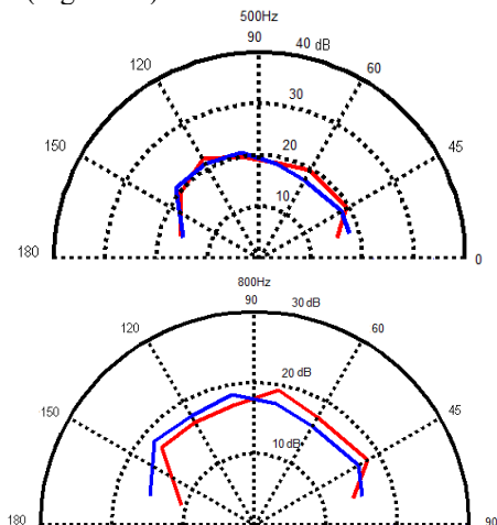
Figure 13 Polar plot of scattered energy (in dB) obtained from simulation (—) and measurements (—) with 22.5° of step for 500Hz and 800Hz and 45° of angle of incidence.
