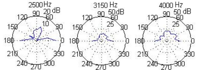
Figure 7. Polar responses of scattered energy (in dB) for Heather plants for 90° speaker incident angle.
