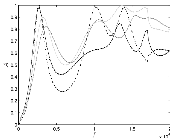
Figure 3: Absorption coefficients for different type of inclusions when the porous slab is excited at normal incidence. Results are computed with the MFS (lines) and with the FEM (dots). The type of inclusion is identified by the color: horizontal ellipse (black), vertical ellipse (dark grey), oblique (light grey), circle (dash-dot).
