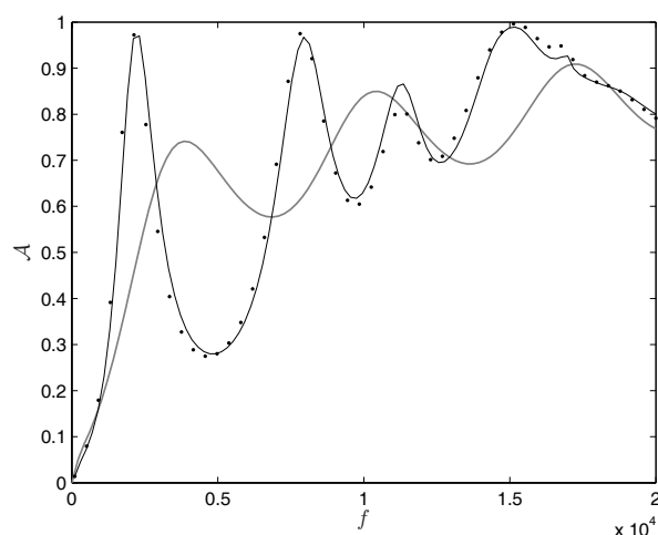
Figure 7: Absorption coefficients for the letter ‘M’ when the porous slab is excited at normal incidence. Results are computed with the MFS (lines) and with the FEM (dots). The grey line refers to the homogeneous slab.
