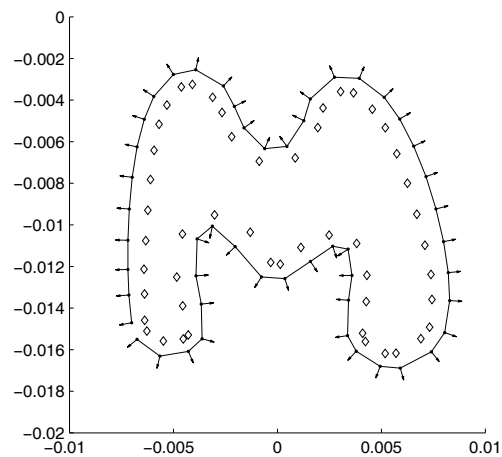
Figure 6: ‘M’-shaped rigid inclusion.
