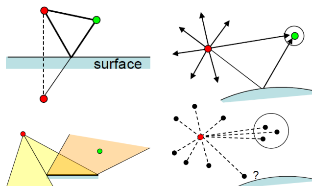
Figure 2: Image source (top, left), ray-tracing (top, right), beam-tracing (bottom, left), particle tracing (bottom, right).
