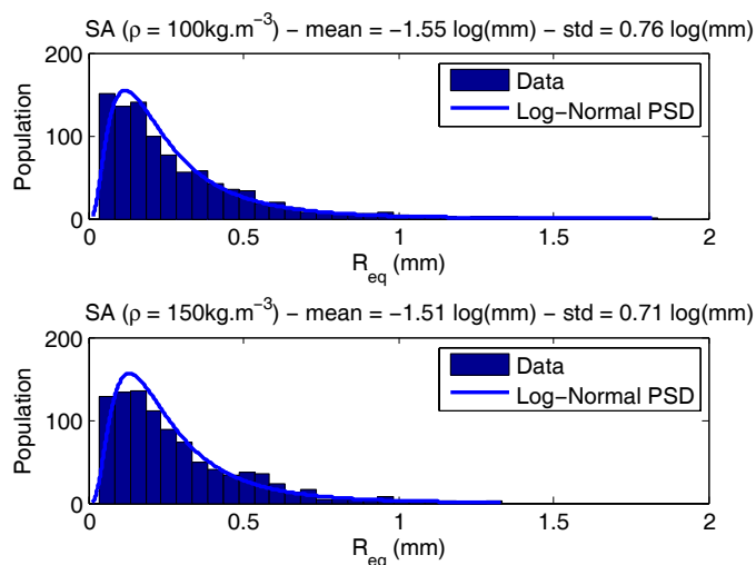
Figure 3: Pore size distribution of shiv S_A , population and associated log-normal distribution
