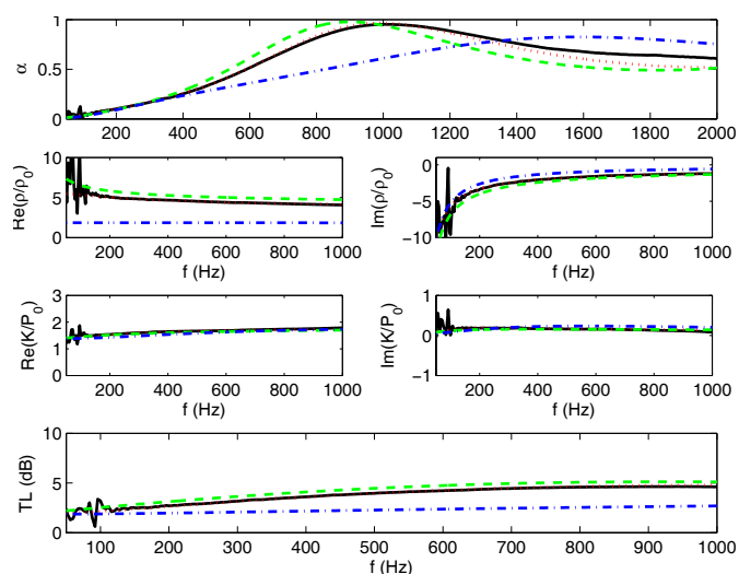
Figure 4: Modelling of shiv S_A - \rho = 150kg.m^{-3} using the general model ( \dots ), the mono-sized spherical model ( -\cdot- ), and the log-normal model ( - - - ), compared to data ( - ).
