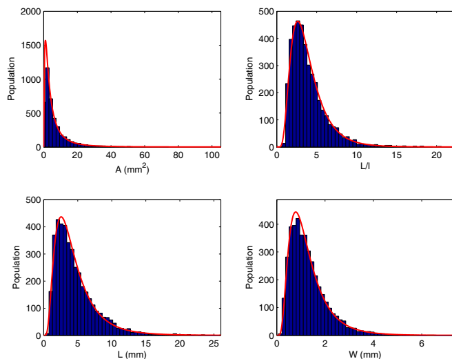
Figure 2: Particle size distribution of shiv S_A , population and associated log-normal distribution
