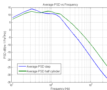
Figure 3: Comparison of the spatial average PSD for the step case and the half cylinder case.
