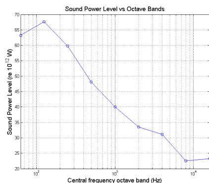
Figure 11: Sound Power level radiated by the panel for the half cylinder case.
