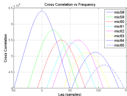
Figure 6: Delay between the microphone number 58 and microphones number 59 to 65 in the arrival of the convected eddies.
