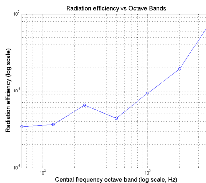
Figure 10: Radiation efficiency in octave bands for the half cylinder case.
