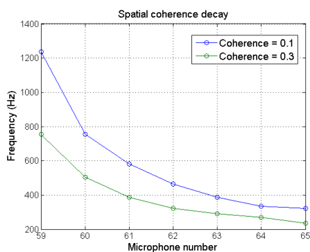
Figure 5: Spatial coherence decay for microphones number 58 to 65 for values of coherence of 0.1 and 0.3 for the step case.
