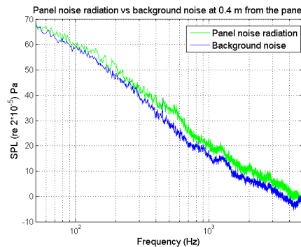
Figure 9: Background noise versus SPL radiated by the panel at 0.4 m from the panel, step case.
