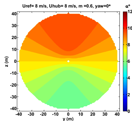
Figure 4: estimated angle of incidence on the rotor disk with a wind shear factor m=0.6
