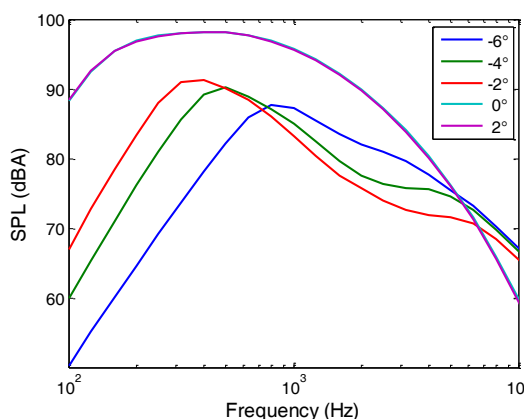
Figure 3: Blade element source spectra as a function of angle of incidence (relative to the stall angle) used by Oerlemans [5] as derived from the BPM model [3]
