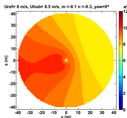
Figure 5: Effect of a local wind gust on the estimated angle of incidence
