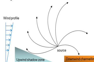
Figure 6: shadow zone due to wind gradients
