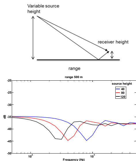
Figure 8: Ground interference dips at 500m range for various source heights
