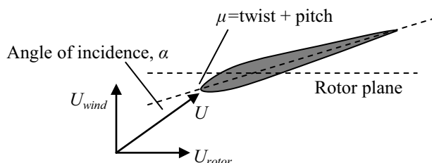
Figure 3: Flow vector geometry showing components due to wind and rotor motion, angle of attack and blade twist
