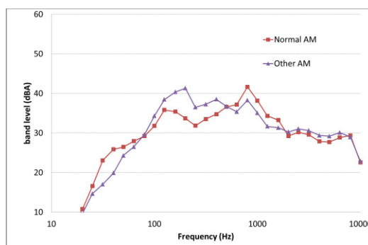
Figure 2: spectra of normal and Other AM for this sample
