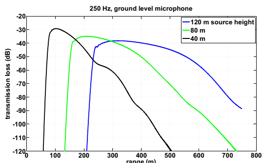
Figure 7 depth of the shadow zone at 250 Hz as a function of source height
