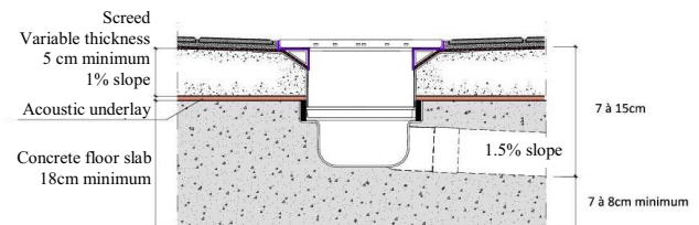
Figure 6: Mounting example of a floor drain with a concrete floating screed [1].
