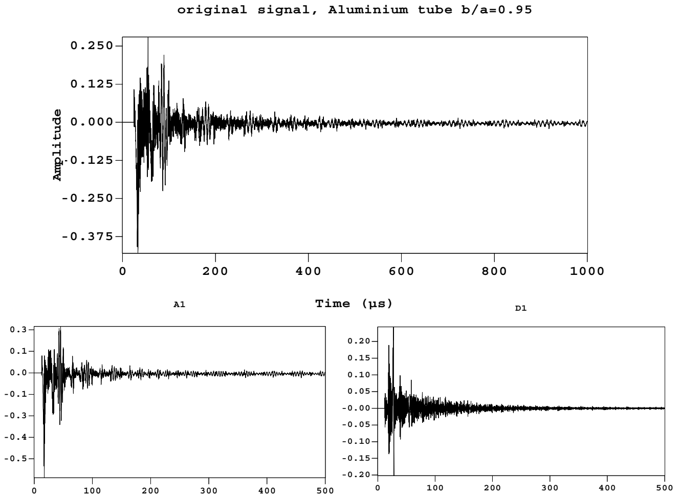
Figure. 6: Filter bank associated with the Multiresolution analysis, approximation coefficients A_{p1} (left) and Detail coefficients D1 (right) with the scaling function and the Daubechies wavelet the order 8
