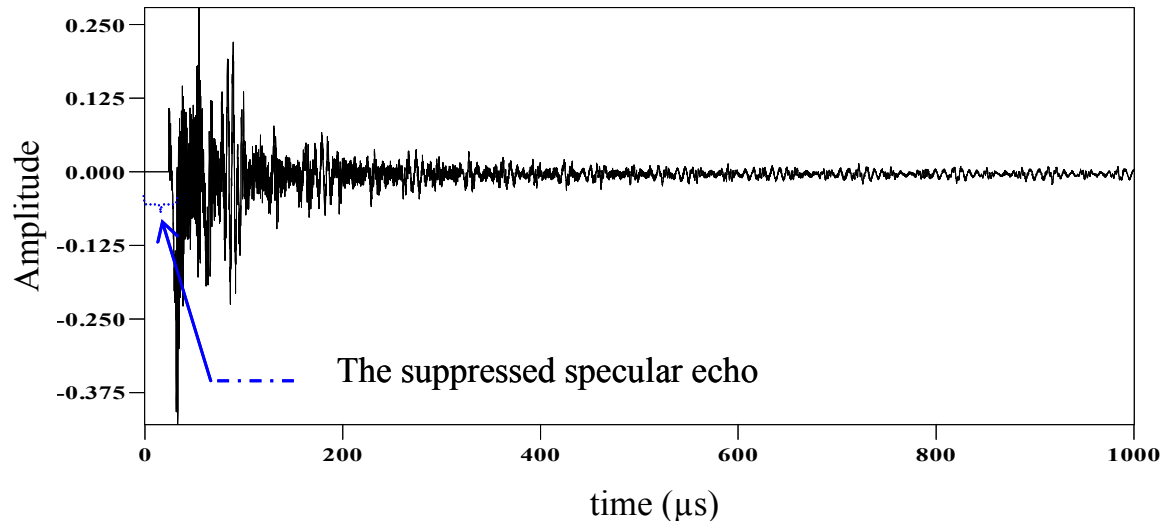
Figure. 3: Temporal signal of an aluminum tube b/a=0.95 , with suppressed specular echo.
