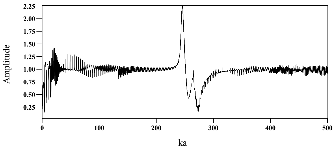
Figure 2: Backscattering spectrum of an air-filled aluminum cylindrical shell immersed in water, b/a = 0.95 , a=3\text{cm}
