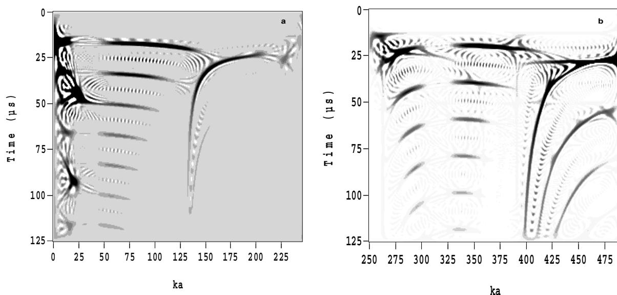
Figure. 7 : SPWV images of the approximation Ap1 (a) and the detail D1 (b)
