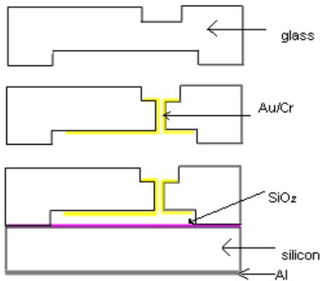
Figure 3: Principal technology steps for the fabrication of the bulk acoustic wave electrostatic resonator: – 1 fabrication of the gap and the protection groove for anodic bonding – 2 manufacturing the via and metallisation for contacting the electrode within the gap – 3 anodic bonding and top side metallization
