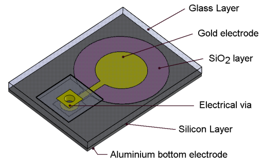
Figure 5: Detailed scheme of the internal structure of the resonator
