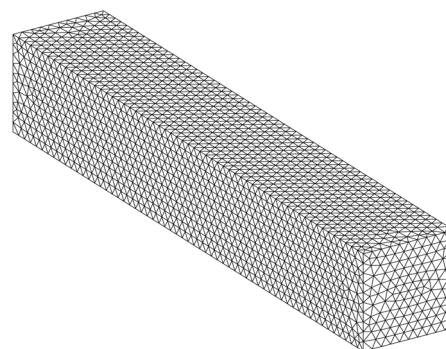
Figure 6: Meshed skin of the second test example (1mx1mx4m parallelepiped filled up with air)
