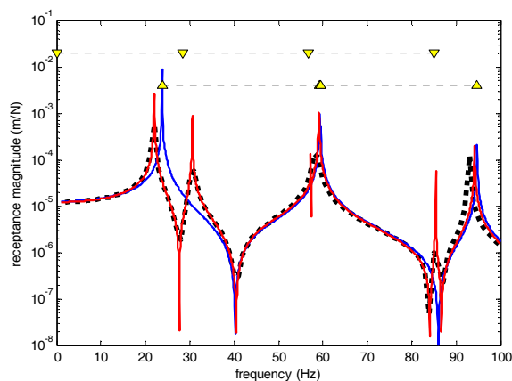
Figure 8: [0,100Hz]-pointwise receptance on an aluminium plate coupled with an acoustic parallelepiped : hf method (-), exact (...), in vacuo (-); acoustic (v) and structural (^) frequencies.
