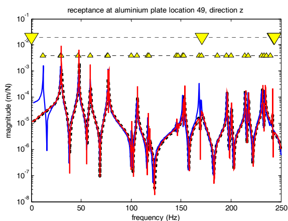
Figure 4: [0,250Hz]-pointwise receptance on an aluminium plate coupled with an acoustic cube : hf method (-), exact (...), in vacuo (-) ; acoustic (v) and structural (^) frequencies
