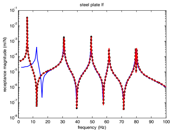
Figure 3: [0,100Hz]-pointwise receptance on a steel plate coupled with an acoustic cube : added stiffness and mass (-), exact (...), in vacuo (-)
