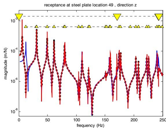
Figure 5: [0,250Hz]-pointwise receptance on a steel plate coupled with an acoustic cube : hf method (-), exact (...), in vacuo (-) ; acoustic (v) and structural (^) frequencies
