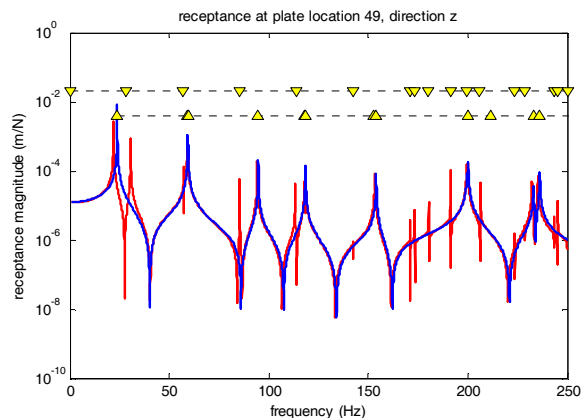
Figure 9: [0,250Hz]-pointwise receptance on an aluminium plate coupled with an acoustic parallelepiped: hf method (-), in vacuo (-); acoustic (v) and structural (^) frequencies.
