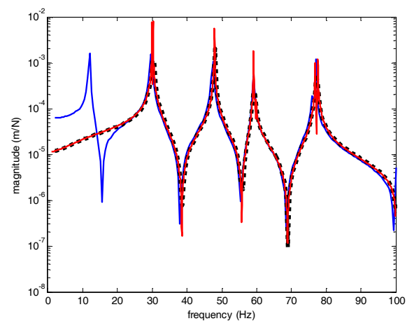
Figure 2: [0,100Hz]-pointwise receptance on an aluminium plate coupled with an acoustic cube : added stiffness and mass (-), exact (...), in vacuo (-)
