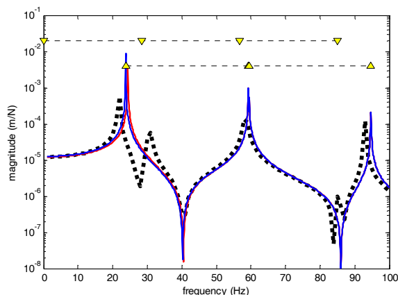
Figure 7: [0,100Hz]-pointwise receptance on an aluminium plate coupled with an acoustic parallelepiped: added stiffness and mass (-), exact (...), in vacuo (-); acoustic (v) and structural (^) frequencies.
