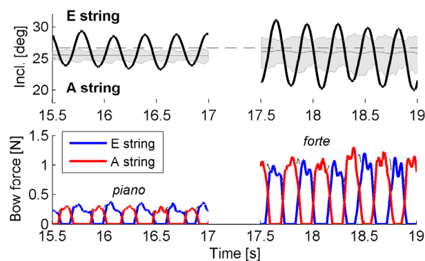
Figure 7: Playing test: circular bowing patterns across two strings, played piano (left) and forte (right).
