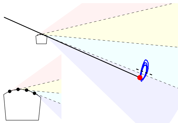
Figure 1: Fixed string positions at the bridge and string crossing angles. The example is a demonstration of that the string crossing angle is not always accurately predicted for stopped strings.
