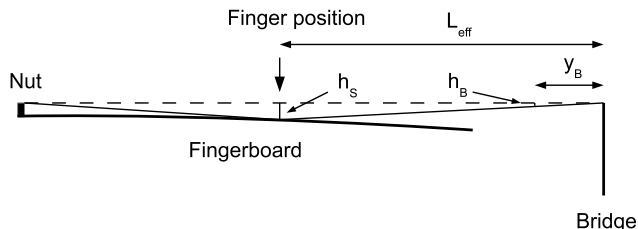
Figure 2: Geometric model of fingerboard (exaggerated proportions).
