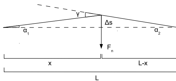
Figure 4: Transverse displacement of the loaded bow-hair ribbon (or string).
