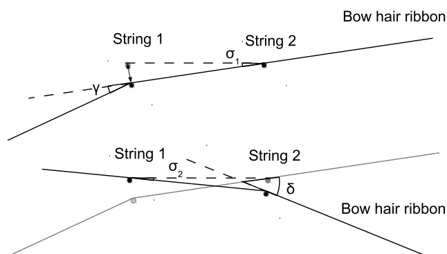
Figure 3: Geometric string transition model (exaggerated proportions).
