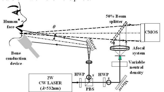
Figure 3: Experimental setup
