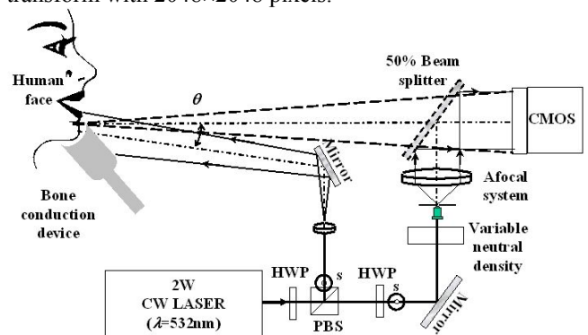
Figure 3: Experimental setup
