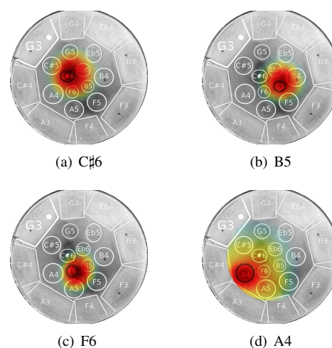
Figure 4: TR FSM imaging and localization of radiating sources when struck by panist
