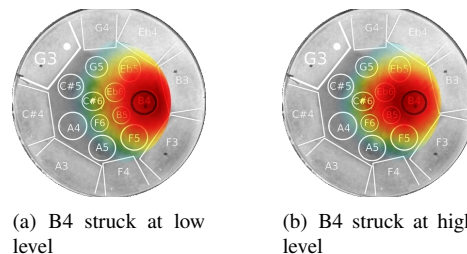
Figure 7: TR imaging and localization of radiating sources when B4 is struck (a) at low level (b) B4 at high level
