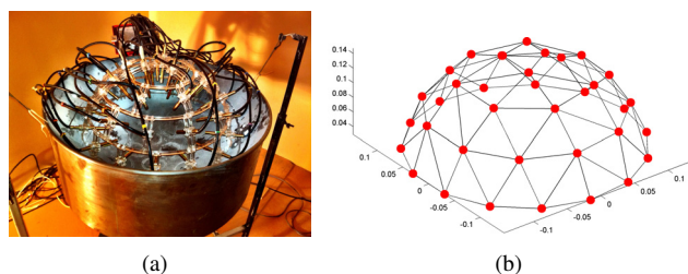
Figure 2: (a) Double-layered hemispherical TRM placed on the steelpan in a reverberating room - (b) Geometry of the TRM: red dots represent the position of each pressure-pressure (p-p) probes on the antenna
