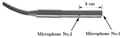
Figure 3: Pressure-pressure probe used in the TRM
