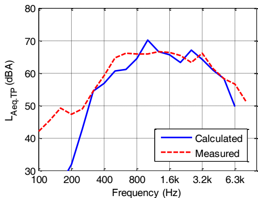
Figure 10: Calculated and measured passby noise spectrum for a 4 car EMU at 80 km/h.
