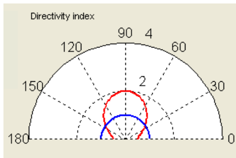
Figure 3: Composite directivity index from combination of monopole and dipole (red line). Monopole (directivity index = 1) as comparison (blue line).
