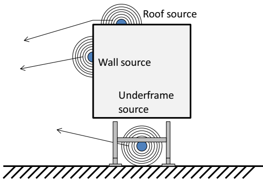
Figure 2: Location of sources for exterior radiation
