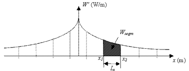
Figure 5: Distribution of track sound power into finite segments based on the track decay rate, The wheel-rail contact is located at x=0 .
