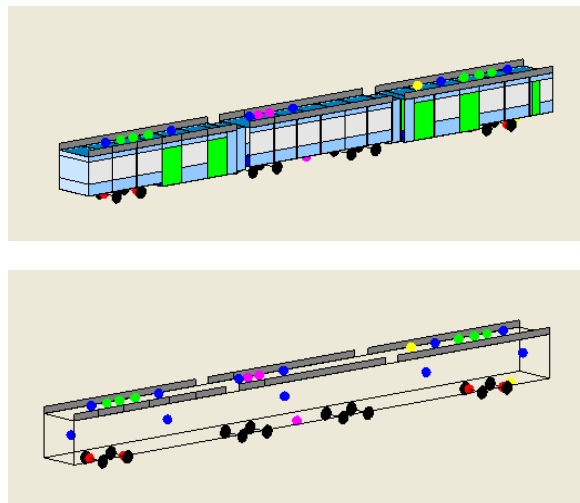
Figure 1: Two views of a BRAINS train model: interior noise analysis (top), exterior noise analysis (bottom). The coloured dots represent point sources.
