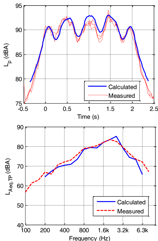
Figure 11: Comparison between measurements and calculation with calibrated model at 190 km/h. Passby noise time history (top), L_{Aeq,TP} spectrum (bottom).
