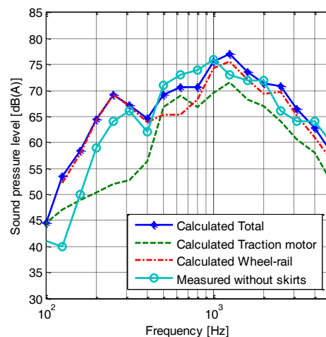
Figure 9: Passby noise calculation (60 km/h) with BRAINS for tram with full set of roughness data (see [7] for details).
