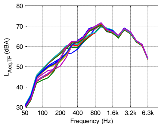
Figure 8: Calculated passby noise spectrum for a range of ground parameter variations. Ground level 0.5-1.5m below top of rail, flow resistivity 100-1000 rayls.
