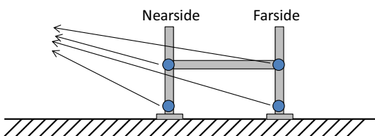
Figure 4: Radiation from wheel-rail sources. Nearside wheel assumed transparent for radiation to the wayside.
