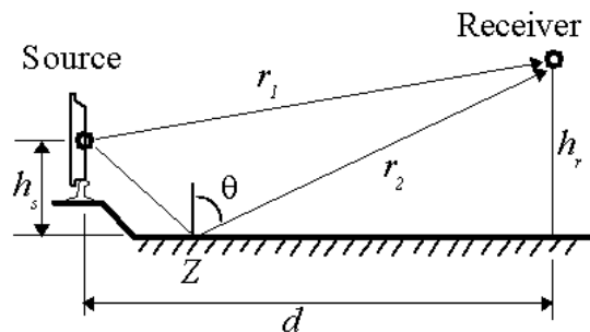
Figure 6: Ground reflection model.
