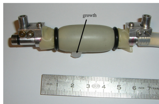
Figure 8: Picture of one vocal fold replica with artificial growth glued.
