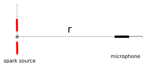
Figure 1: The calibration method is based on the measurement of N -waves at distances r from tens of centimeters to 1.5 \text{ cm} from a spark source.
