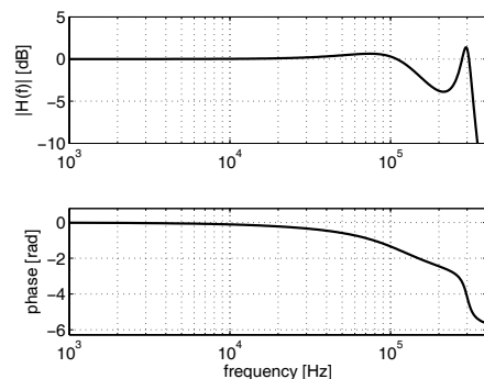
Figure 3: Microphone frequency response. Top: Amplitude response in dB ref. 1 mV/Pa, bottom: Phase response in rad.
