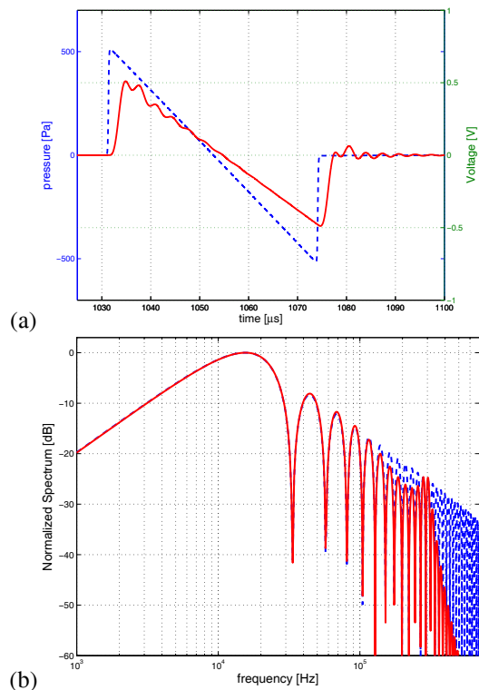
Figure 2: Waveforms and corresponding spectra at 356 mm from the spark source. Blue line: Pressure waveform; Red line: microphone output (microphone frequency response given in figure 3).
