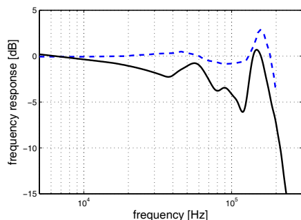
Figure 7: Frequency response of a 1/8 inch condenser microphone (dB, ref. low frequency sensitivity). Black line: estimated frequency response using the proposed method. Blue dash line: frequency response from the calibration chart (electrostatic actuation method).
