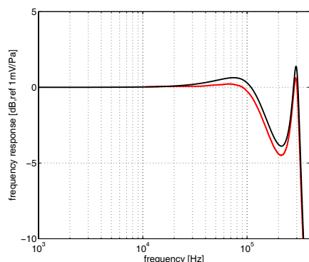
Figure 6: Red line: Amplitude of the frequency response |\tilde{H}(f)| = |V(f)/P_{th}(f)| obtained from a series of recordings at 15 different positions r . Black line: target response |H(f)| given in figure 3.
