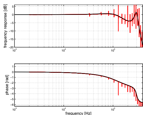
Figure 5: Frequency response \tilde{H}(r, f) = V(f, r)/P_{th}(f, r) estimated from measured and simulation data at the distance r = 356 mm from the spark source.
