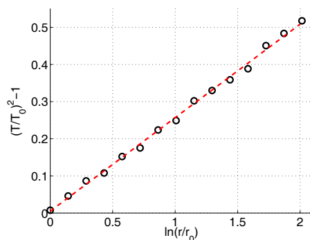
Figure 4: Plot of the evolution of the half duration T with the propagation distance in order to estimate the initial pressure level at the distance r_0 .
