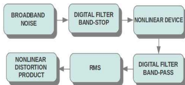
Figure 1: Measuring circuit
